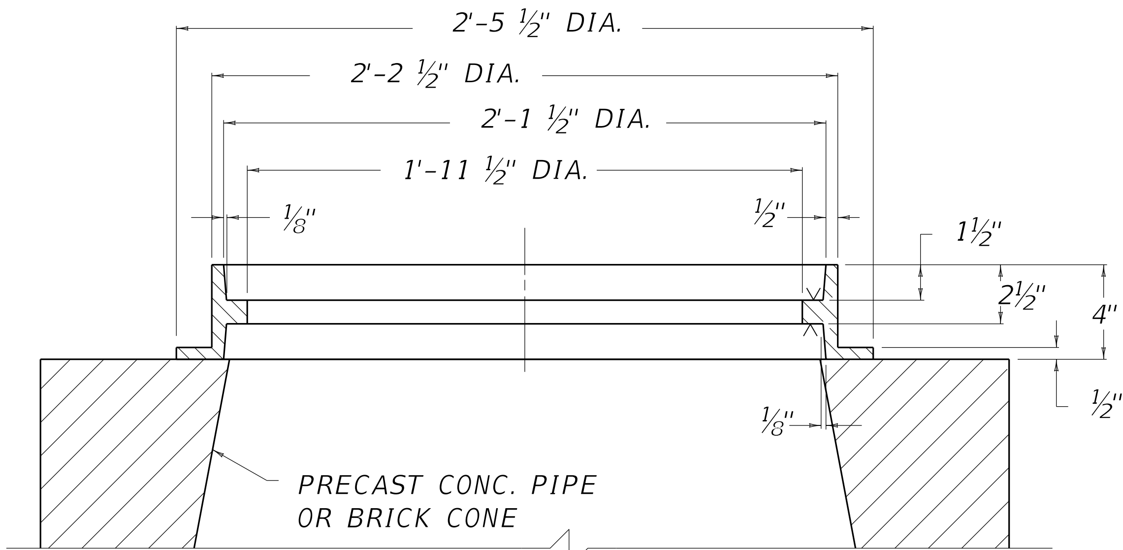
SECTION OF FRAME WHEN USED WITH MANHOLES
