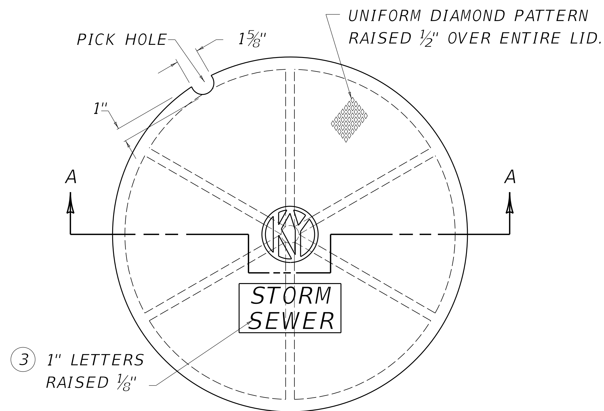
PLAN VIEW
